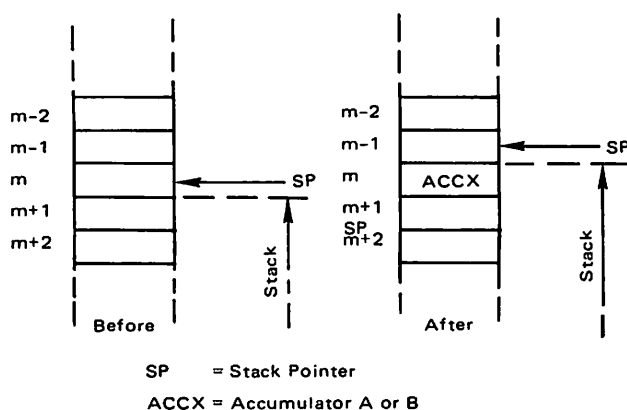
FIGURE 3-5. Data Storage in the Stack
